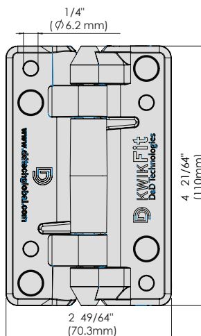
KFP No spring, plain pivoting
