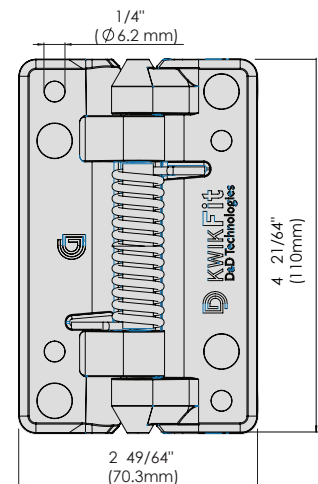
KFS Self-closing, fixed tension
